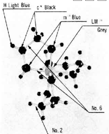
trisethylenediaminecobalt (III) salt [D]
