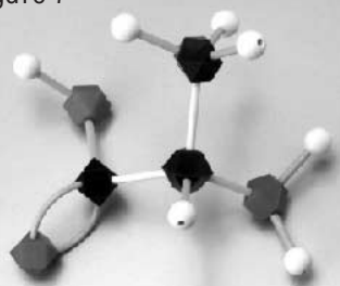
L - alanin ( all set )
