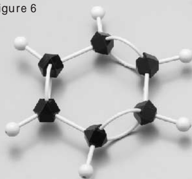
benzene ( 1000,1001,1002 )
