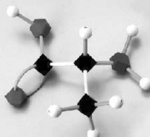
D - alanin ( all set )
