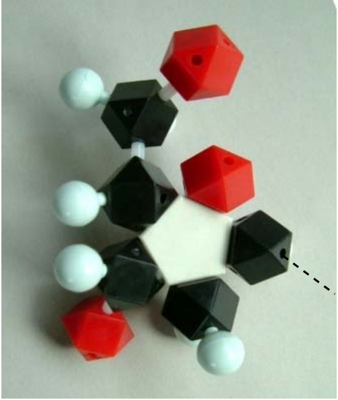
3' Deoxyribose
