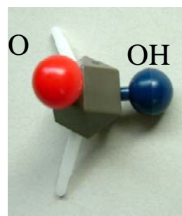
Phosphate
